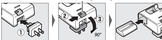
Lichtnetadaptervergrendeling
